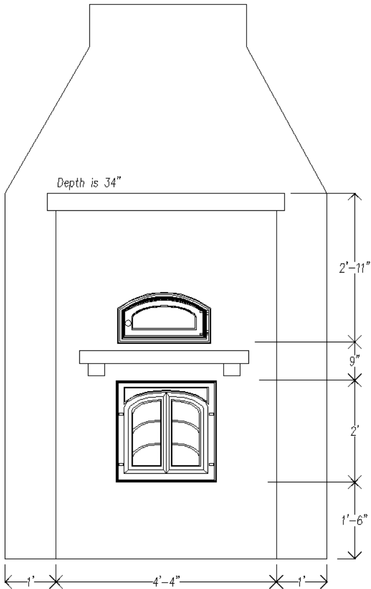
Figure 1 Dimensions of finished fireplace
