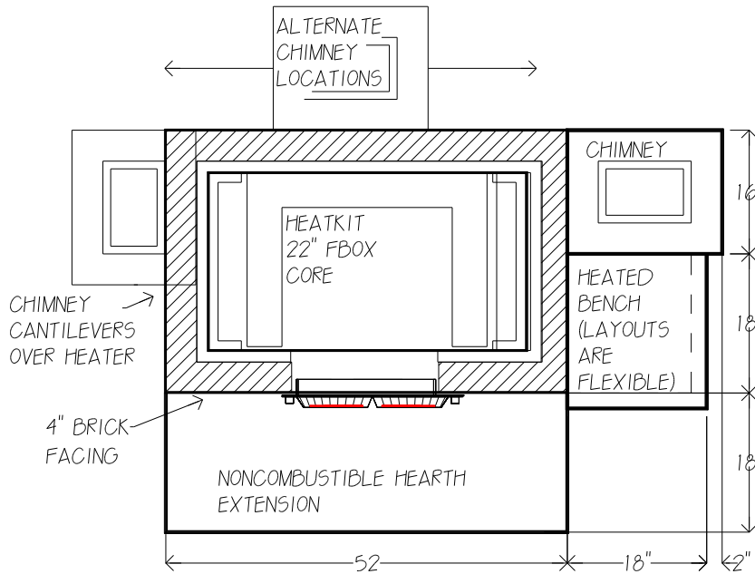
Figure 3. Layout dimensions for determining heater and chimney footprint
