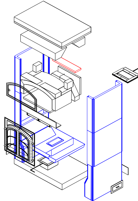
Figure 1. Kit components, exploded view connecting plenum (8) under the firebox. From there the cooled exhaust gases enter the chimney at floor level. The design of the connecting plenum allows the chimney to be connected anywhere at the back or side of the heater without unbalancing the downdraft channels.
