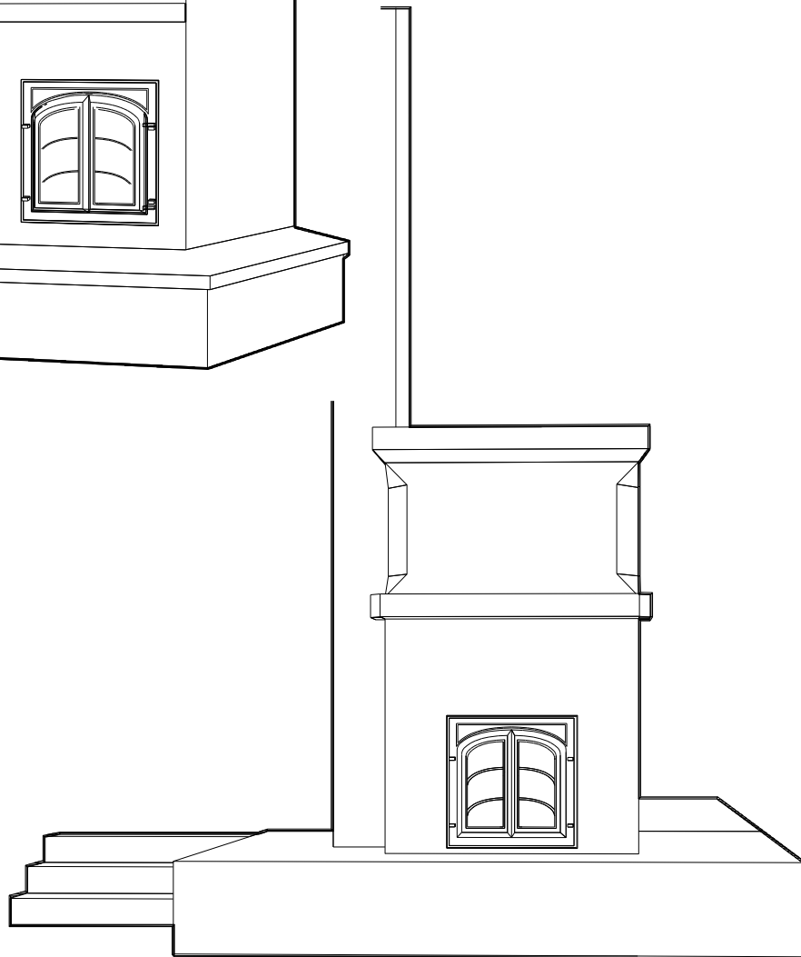
Figure 6. Sunken living room, raised heated hearth
