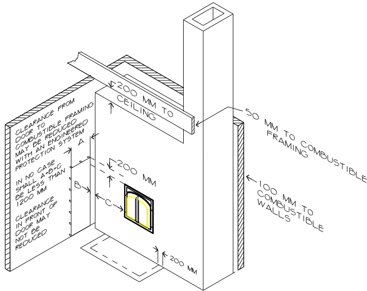
Figure 12. ASTM clearances to combustibles for masonry heaters.
