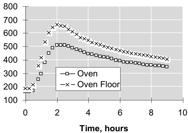
Figure 2. Oven and oven floor temperature cycle
